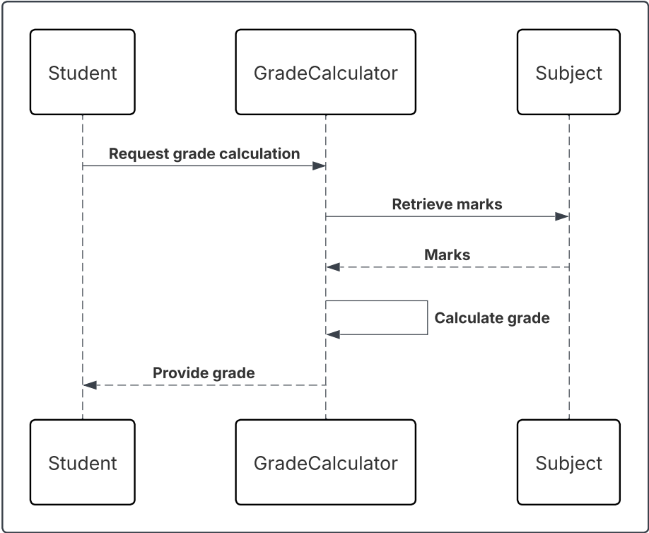
Grade Calculation Sequence Diagram
