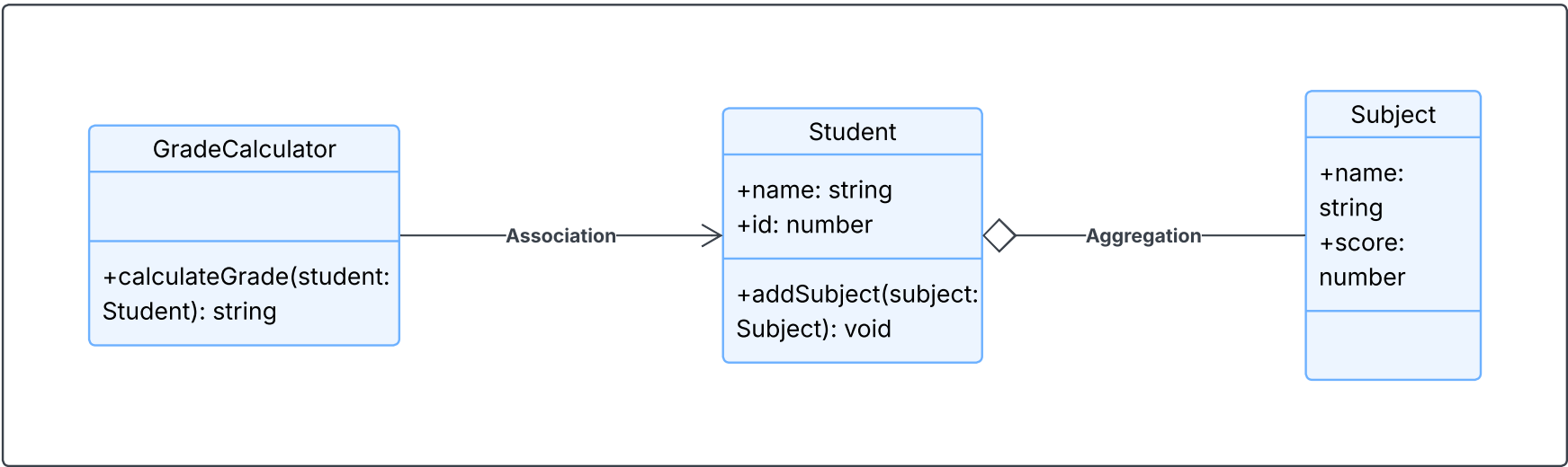
School Results Application Class Diagram
